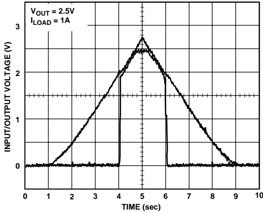
Figure 11. Power-Up/Power-Down
